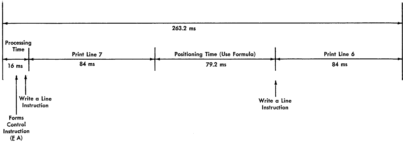
Figure 16. Print Lines 6 and 7 of Each Card
