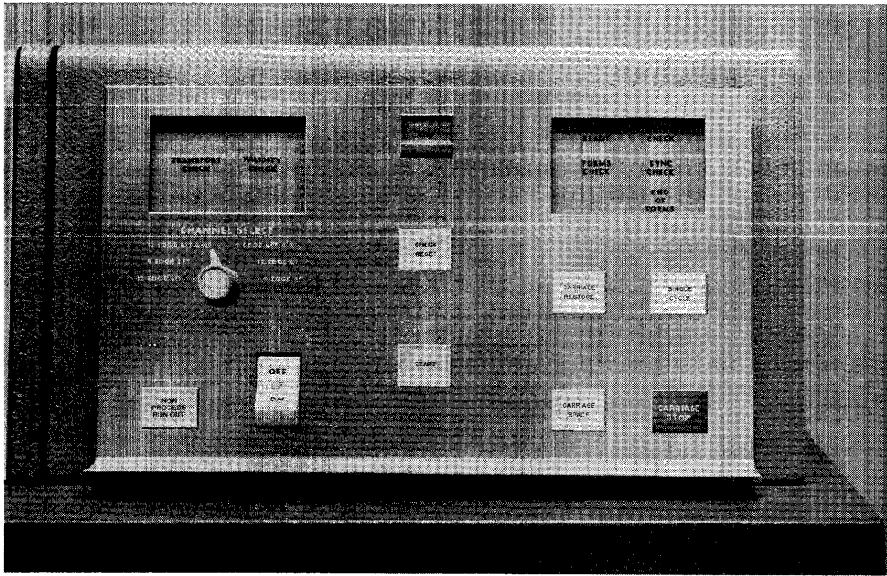
Figure 7. Console, IBM 1404
