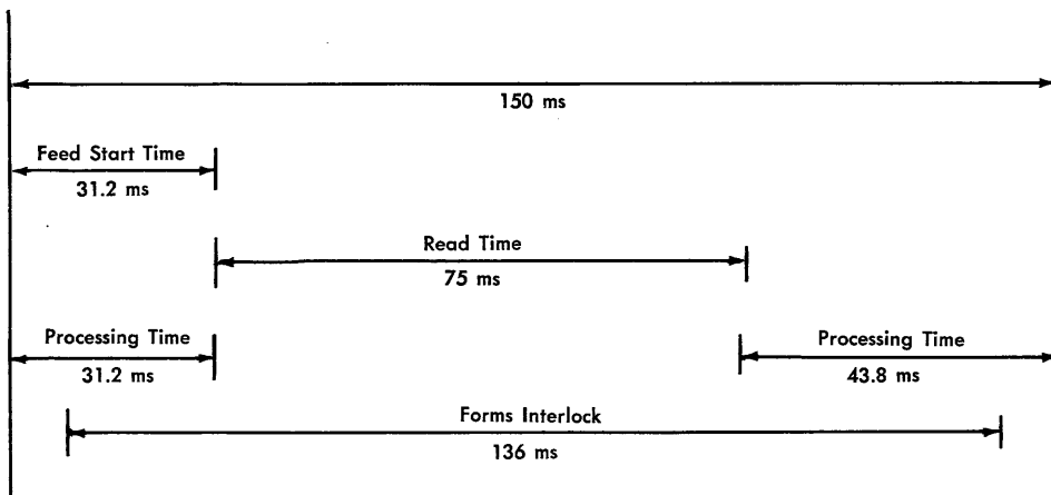
Figure 17. Read Timing Chart, IBM 1404
