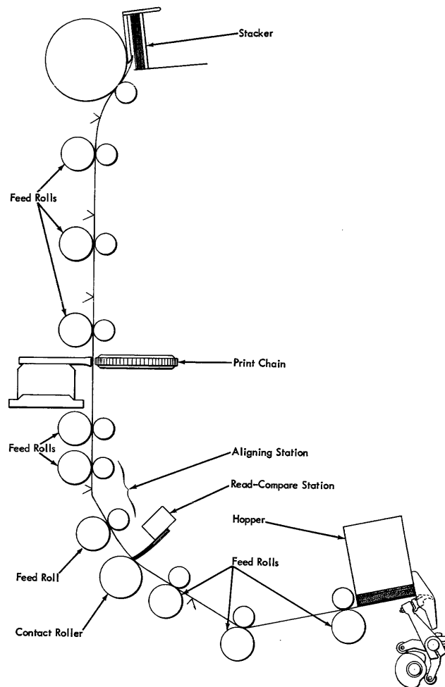
Figure 5. Card Transport Schematic, IBM 1404
