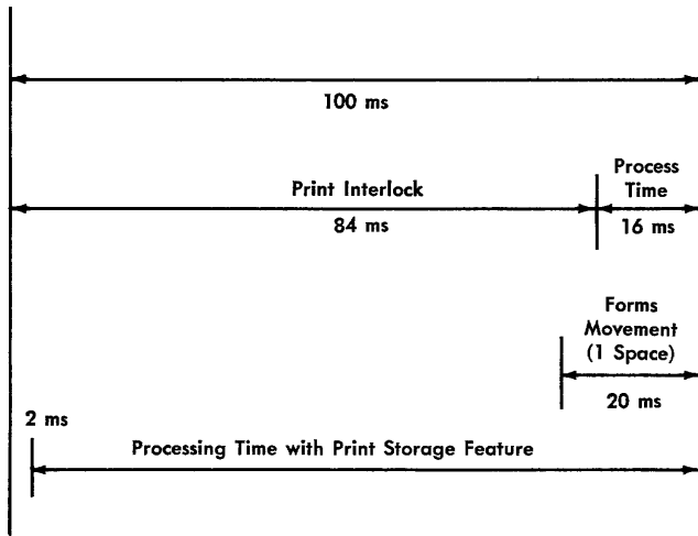
Figure 14. Print Timing Chart
