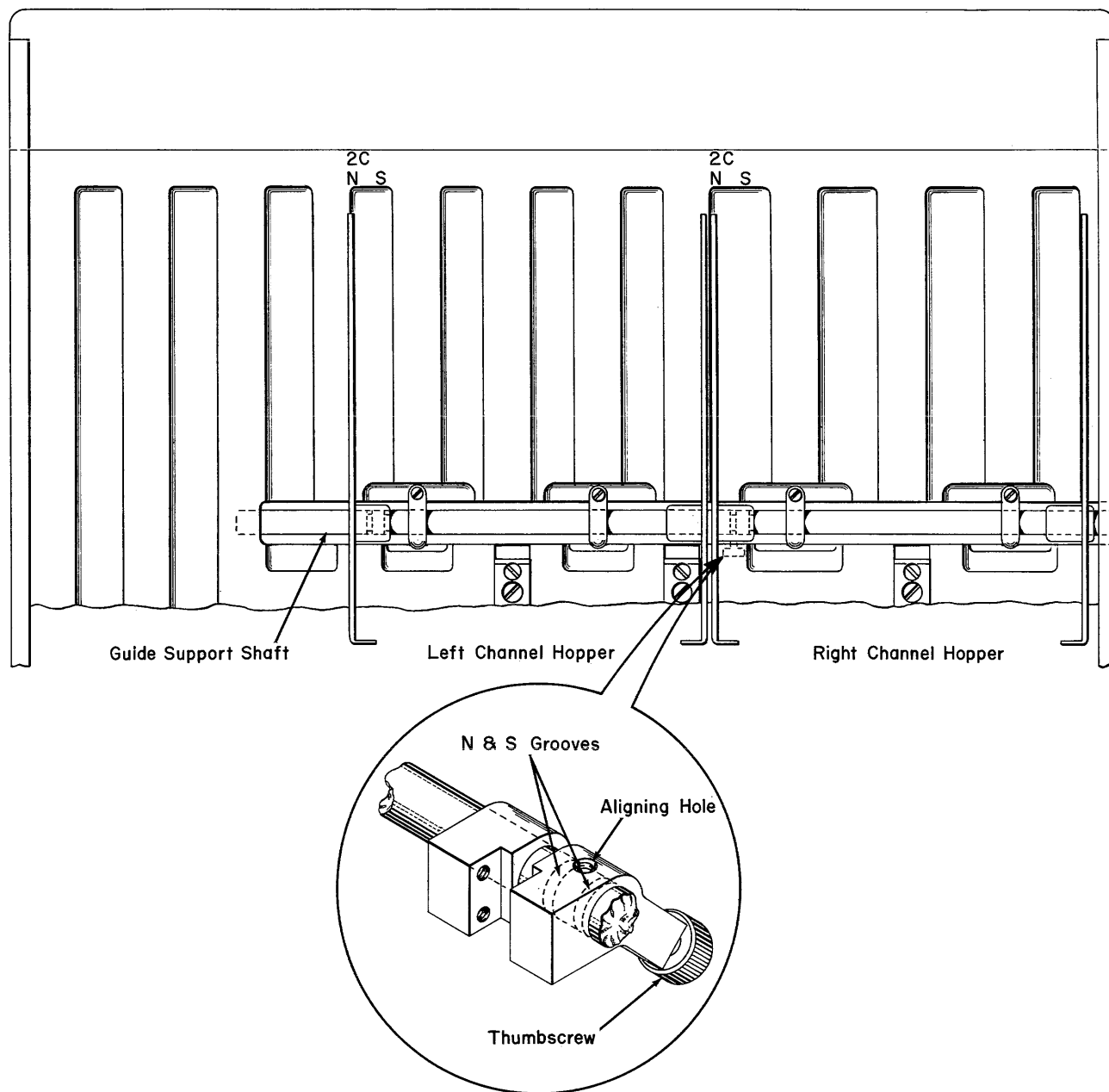
Figure 3. Hopper Side Plate Adjusting Mechanism
