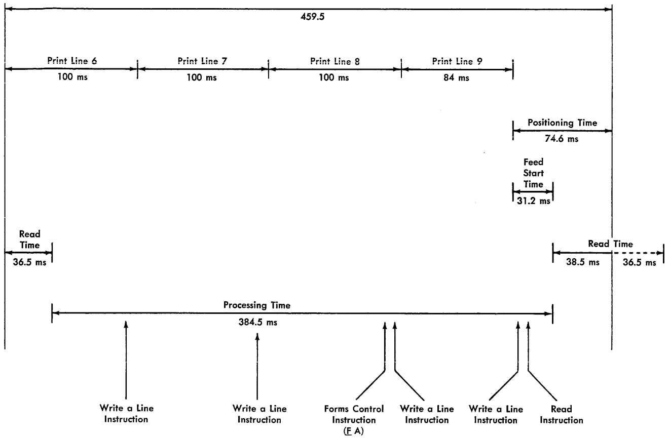
Figure 21. Print (4 Lines) and Read Timing Chart, IBM 1404 (with Print Storage)
