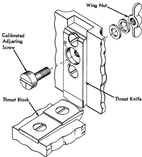
Figure 4. Throat Adjusting Mechanism
