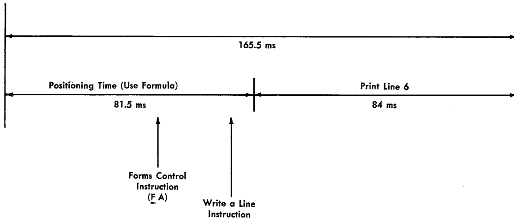
Figure 15. Print Line 6 of Each Card
